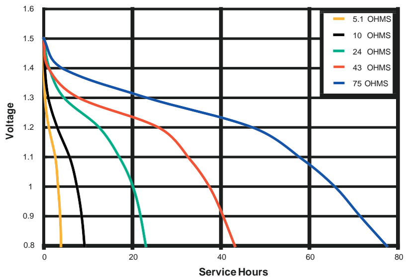
TYPICAL DISCHARGE CHARACTERISTICS AT 21°C
